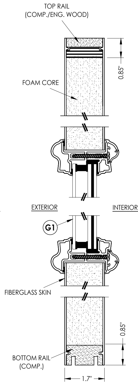
2 3 VERTICAL CROSS SECTION COMPOSITE EDGE SIDELITE PANEL
